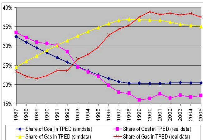
Figure 15: Shares of coal and gas in TPED: simulated vs. real data
