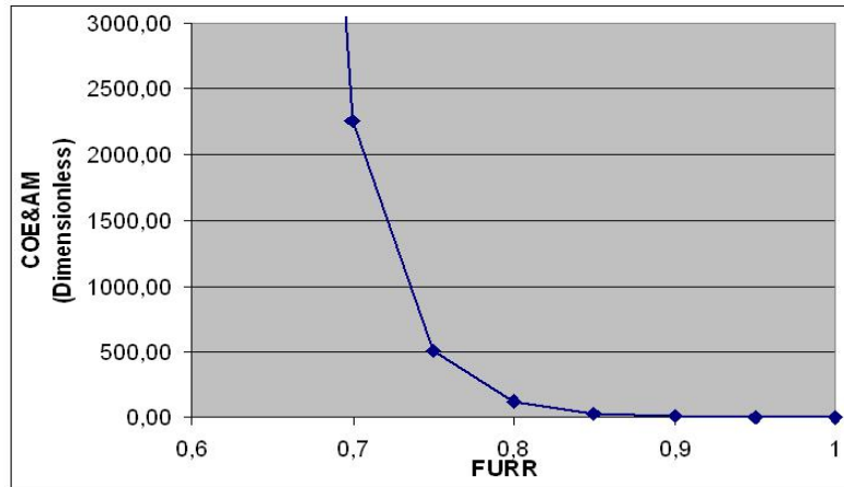
Figure 2: Relationship between FURR and COE&AM
