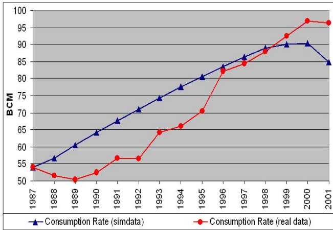
Figure 13: Consumption rate: simulated vs. real data
