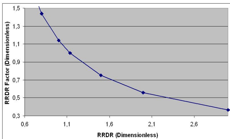
Figure 4: RRDR versus RRDR Factor
