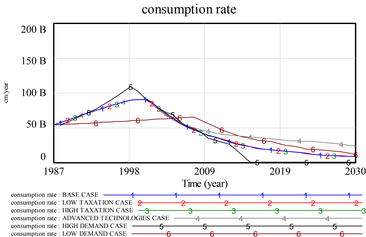
Figure 21: Dynamics of CR in alternative cases
