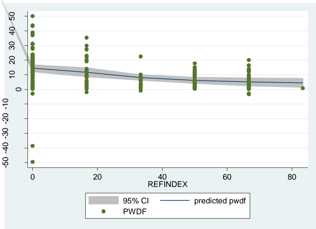
Figure 4.9: Fractional Polynomial Prediction Plot: Total Energy Deficit versus Reform Index 47
