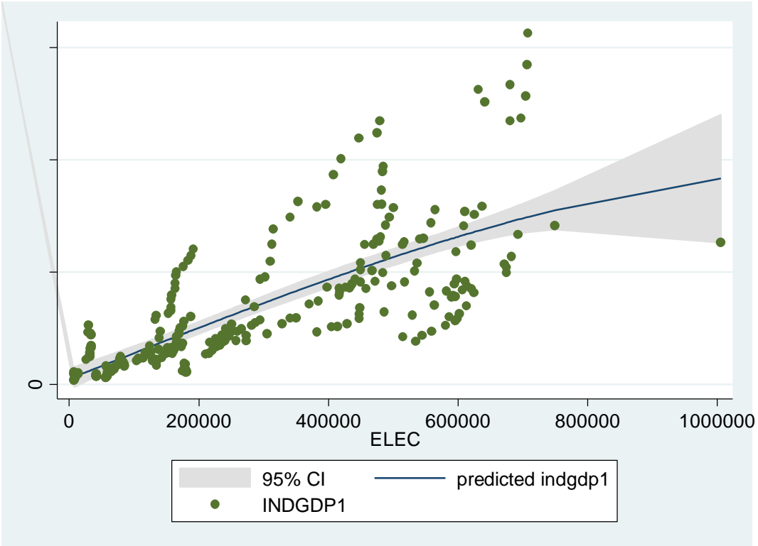
Figure 4.1: Fractional Polynomial Prediction Plot for Electricity Infrastructure versus Total Industrial GDP
