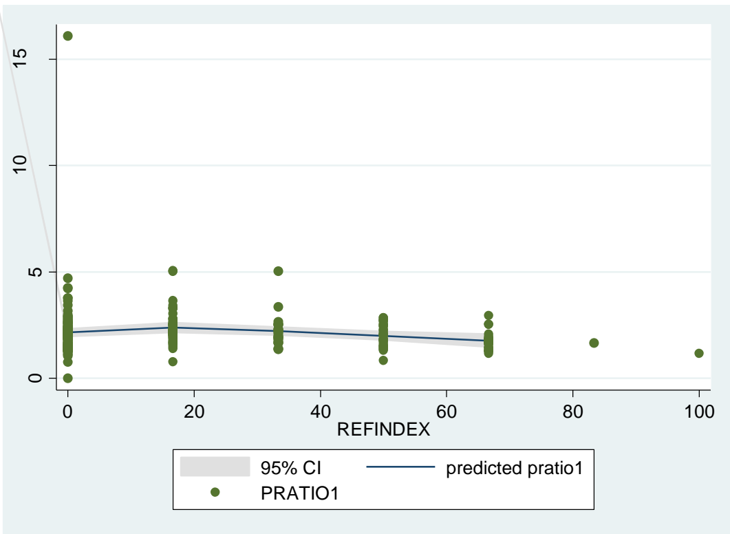
Figure 4.7: Fractional Polynomial Prediction Plot: Ratio of Industrial to Domestic Price versus Reform Index
