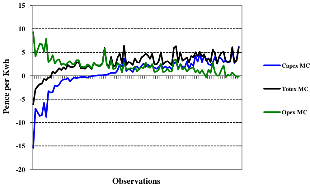
Figure 8. Decomposing marginal cost of reducing electricity distribution losses
