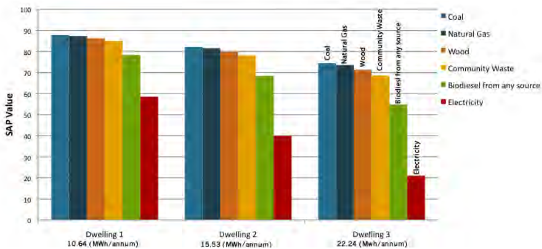
Figure 12: Effect of fuel type on SAP
