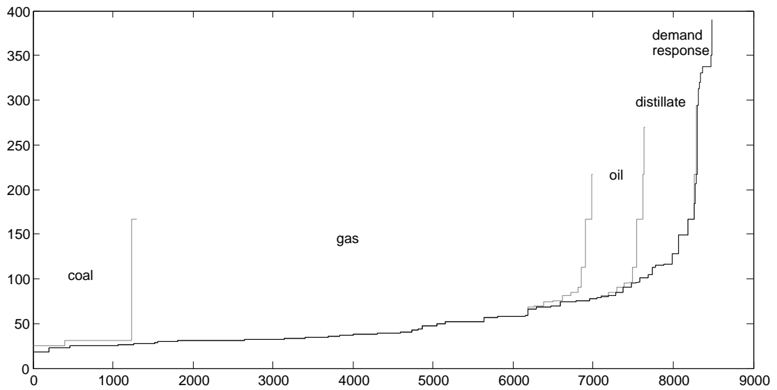
Figure 6: Aggregated representative bid curves by fuel in the SEM in 2015.
