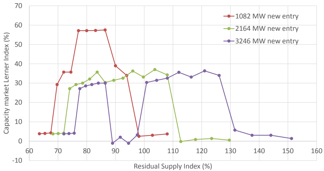
Figure 16: Lerner index in the capacity market vs. Residual Supply Index (RSI) with different amounts of procured capacity. 80 % forward contract share is assumed.
