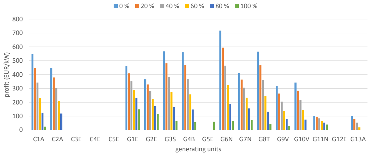
Figure 7: Unit-specific profits with different shares of forward contracts in the energy-only market.
