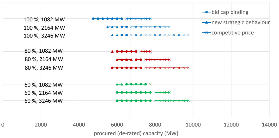
Figure 17: Binding and competitive market results when 60 EUR bid cap is set for incumbent units (except for ESB's coal units). Total capacity restricted by the lower bid cap is 6681 MW.
