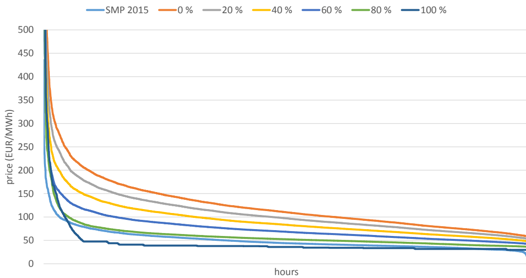
Figure 8: Price duration curves with different shares of forward contracts in the energy-only market.
