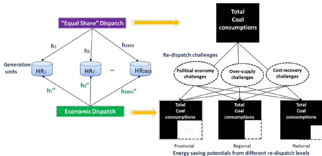
Fig. 1. Research framework
