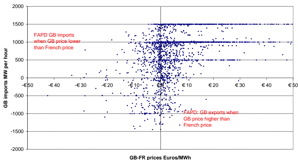
Figure 2. Ex post Net GB imports over IFA vs. day-ahead price differences during 2013.
