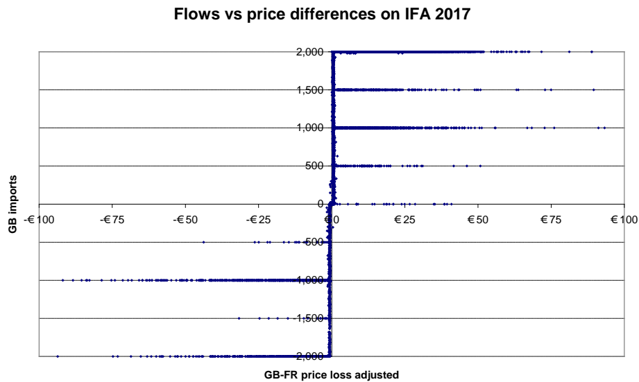
Figure 3. Ex ante scheduled net imports into GB over IFA vs day-ahead price differences, 2017. Source: Prices: N2EX for GB, ENTSO-E for FR, data truncated at +/- €100/MWh. Flows are RTE forecast flows.
