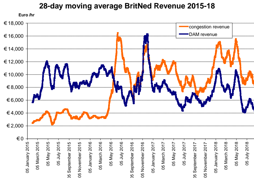
Figure 6. Congestion revenue estimated from DAM prices and recorded congestion revenue. Source: ENTSO-E Transparency platform.
