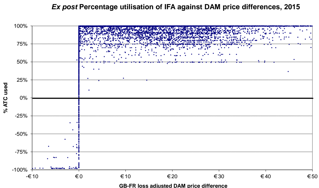
Figure 4. Ex post GB net imports from France as a percent of ATC against the GB minus French (FR) price differences, calendar 2015.
