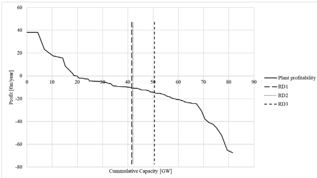
Figure 1: An example of profitability of conventional plants in Germany. Note: “RD1-3” = residual demand for three peak demand hours.
