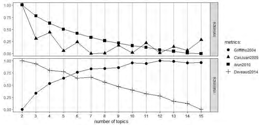
b. Optimal number of topic determination using Lдатuning algorithm
