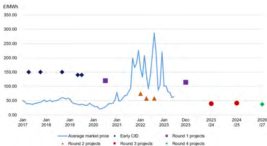
Fig 10. UK market electricity price and CfD strike prices (in 2012 price). Note: CfD supported projects before Jan 2023 are situated at the dates when they commissioned. After that, delivery years (when projects are expected to commission).
