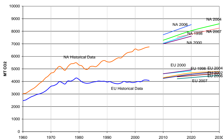
Figure 6: OECD Europe and North American CO 2 emissions & IEA business as usual projections
