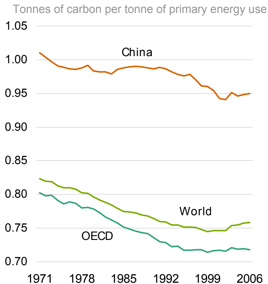
Carbon Intensity
